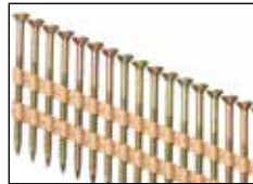
2-1/4" x 0.113 #2 Phillips drive zinc coated
