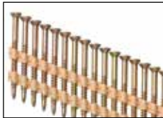
2" x 0.131 #2 square drive zinc coated
